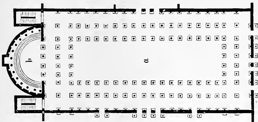
FIG. 130.—GROUND-PLAN OF THE BASILICA ULPIA, ROME.
